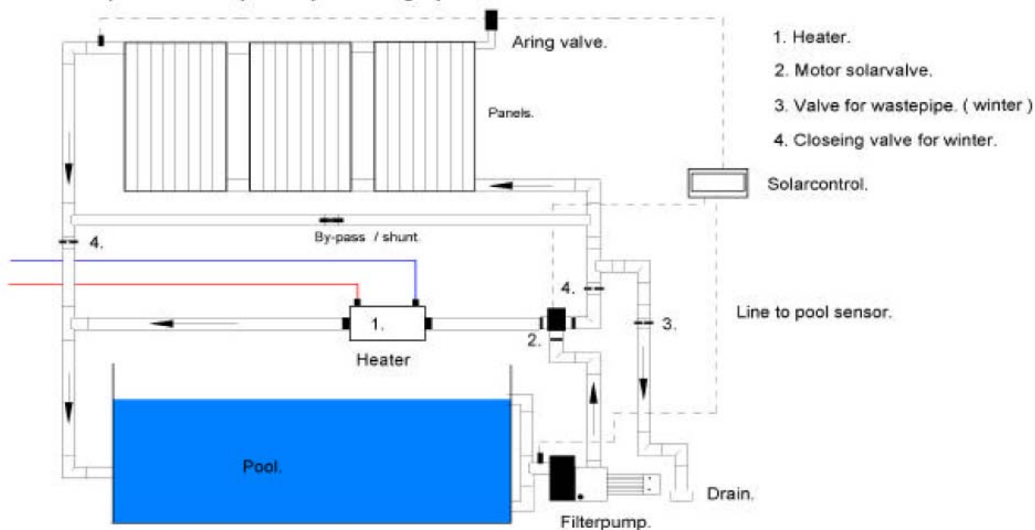
Princip chart for solarpanels up to 5 m. high placement
